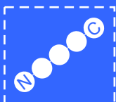
Standard Peptide Synthesis
