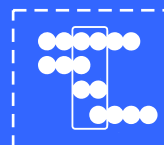
Cosmetic Peptide Synthesis
